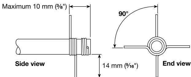
Pinch together (to relax coil) for fitting to probe tip
